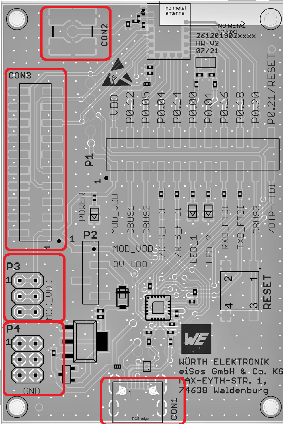
Figure 3: Connectors
