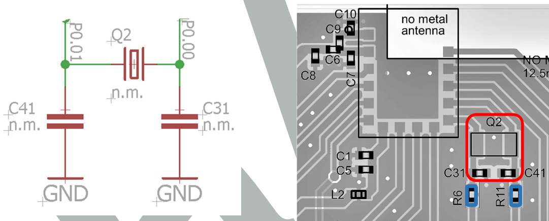
Figure 7: LFXO mounting
