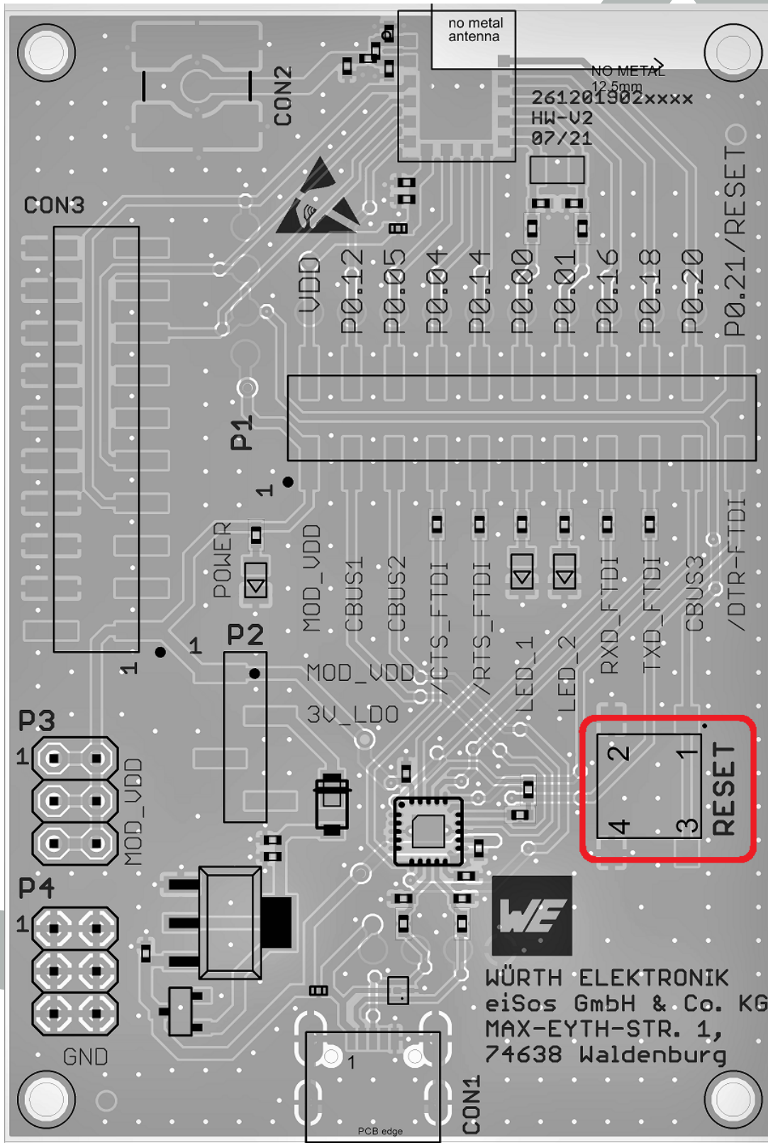
Figure 6: Buttons
