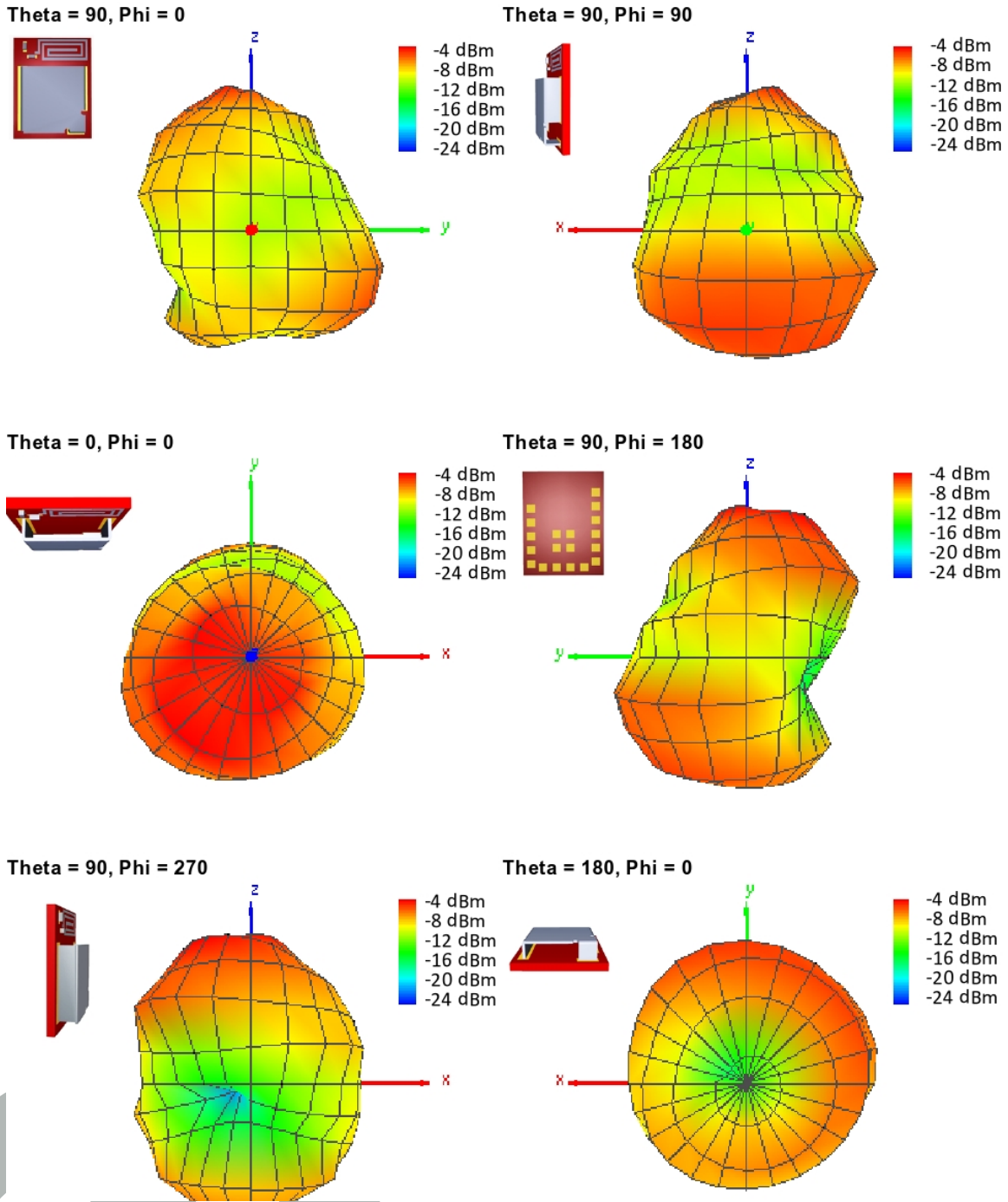
Figure 11: Antenna characteristic from integrated antenna measured on official EV-Board 1
